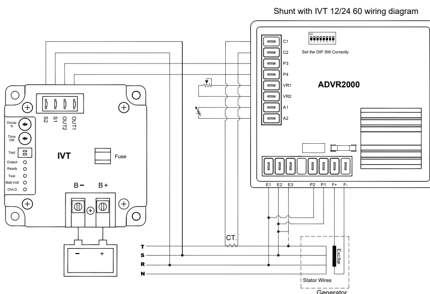
Figure 6 ADVR2000 & IVT-1260 / IVT-2460 Wiring Connection
