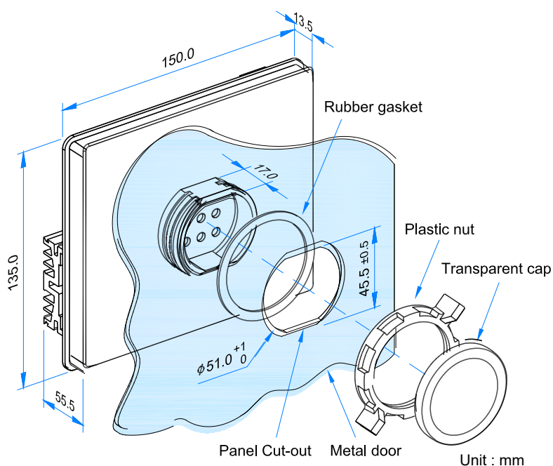
Figure 1 Outline Drawing
